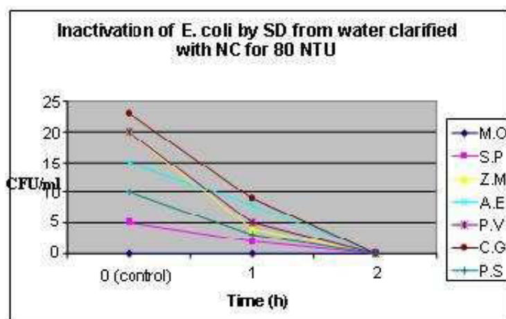
Figure 6: Inactivation of E. coli for high turbid sample.
